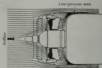
FIGURE 6-45. Engine airflow.
